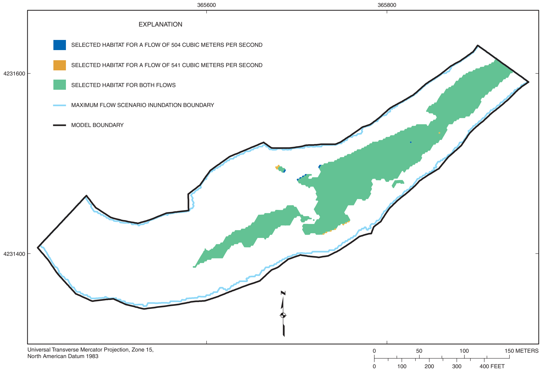
Figure 4-41. Selected habitat area distribution for habitat category 7 (paddlefish) at flows of 504 and 541 cubic meters per second at Marais des Cygnes River site MDC2.
